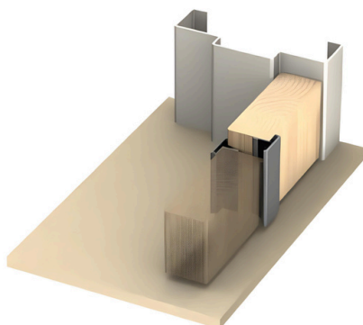
Dual leaf door meeting stile: IS7061si x 2
