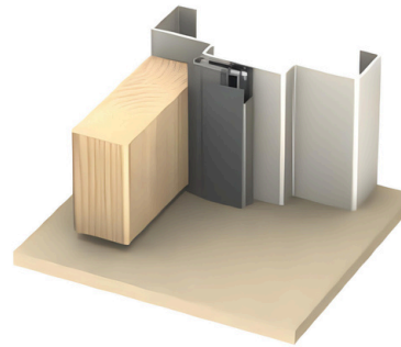
Perimeter seal: IS7087si
