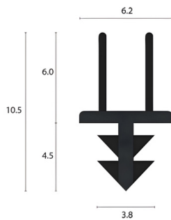
Perimeter seal: IS0511
