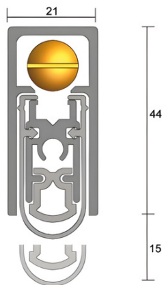
Threshold automatic drop seal: IS8520si
