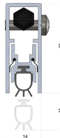
Drop seal: IS8011si
